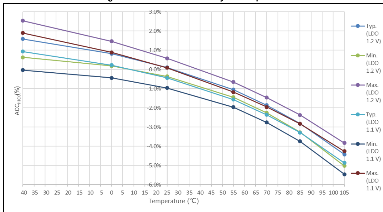
Figure 15. HICK clock accuracy vs. temperature
