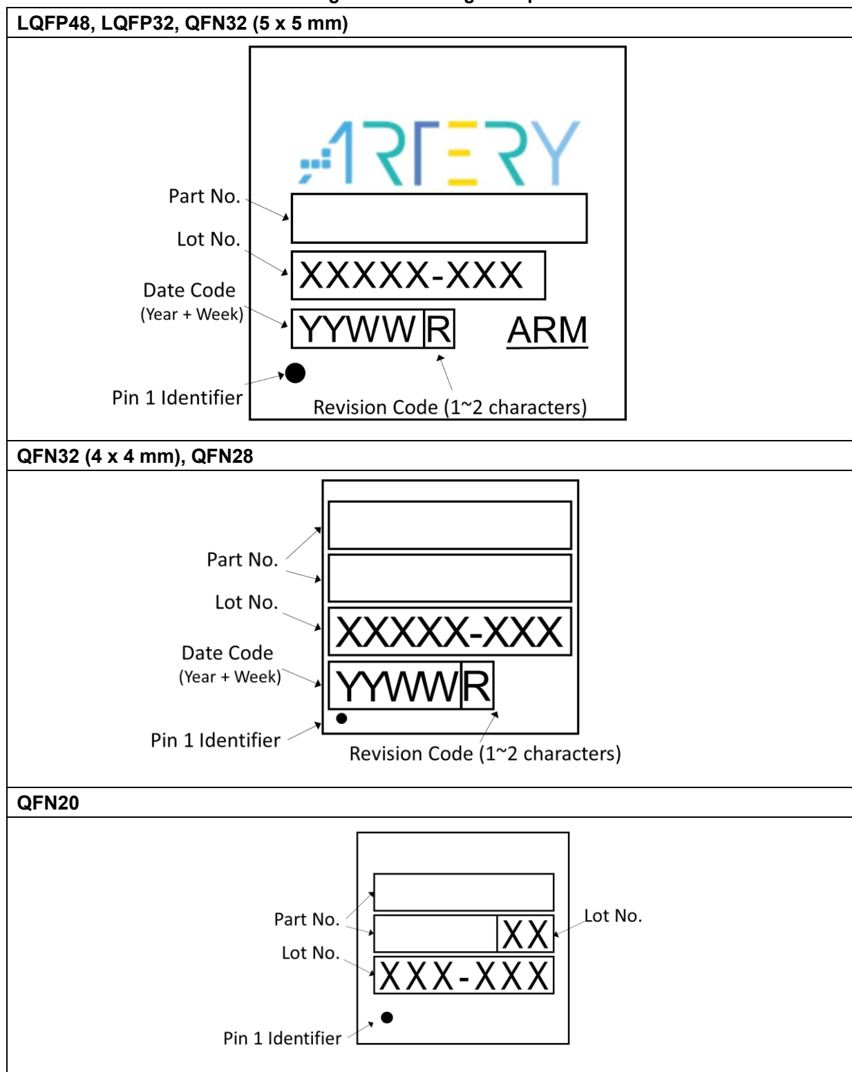
Figure 31. Marking example
