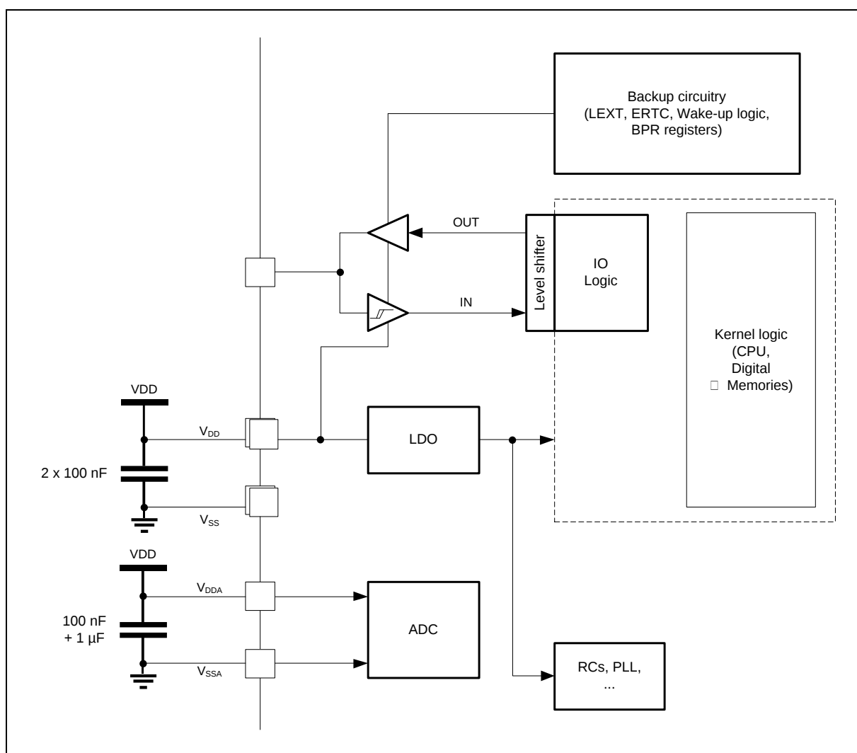
Figure 9. Power supply scheme
