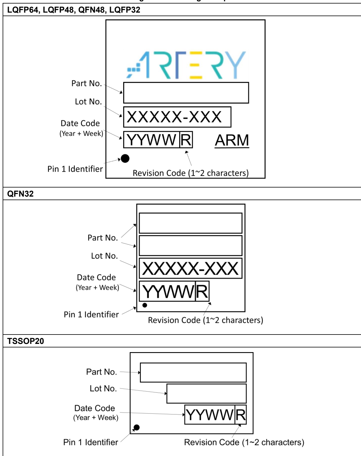
Figure 35. Marking example
