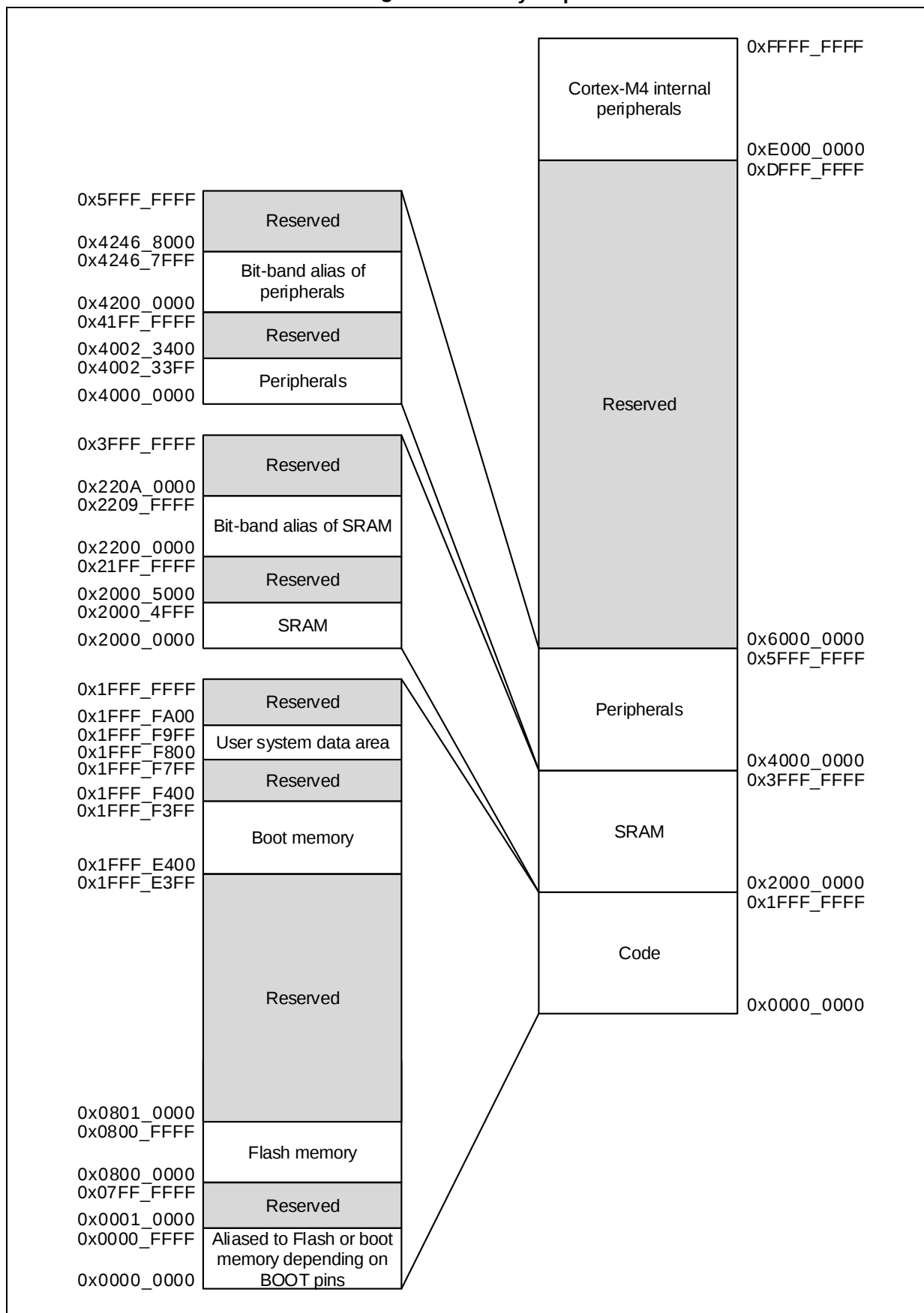
Figure 8. Memory map
